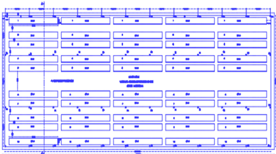
1400 MT. ONION STORAGE SHED PLAN UNIT NO.1
