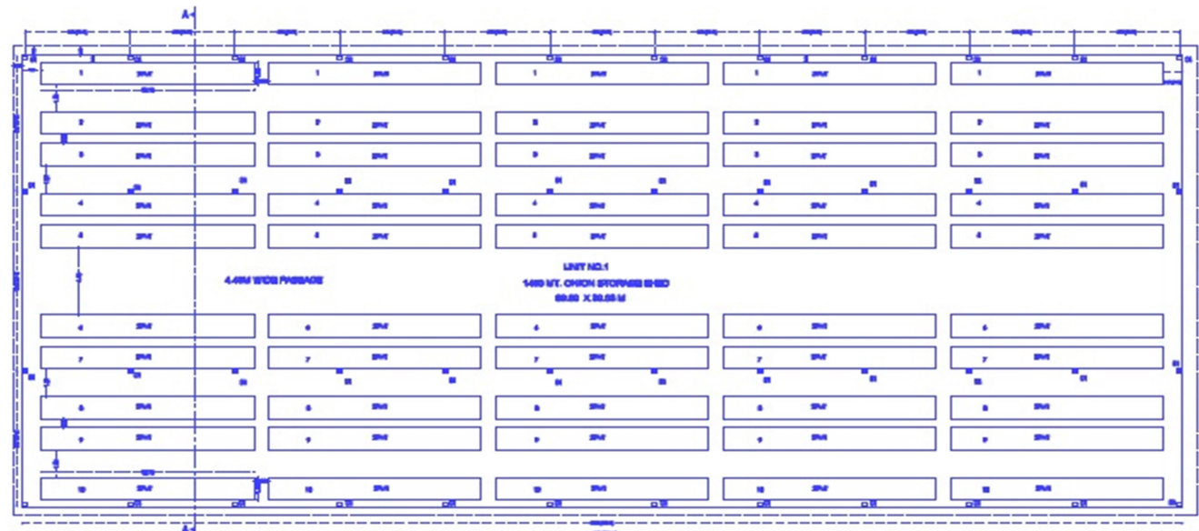
1450 MT. ONION STORAGE SHED PLAN UNIT NO.1
